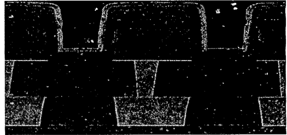
Fig. 4. Thick top aluminum layer and base copper layer used for dual metal inductors.
