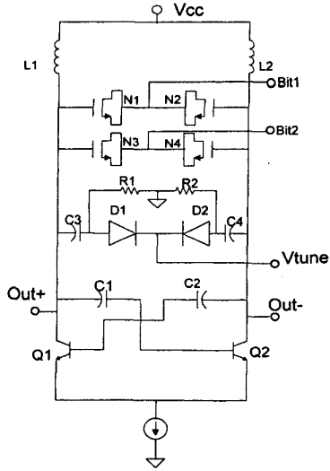
Fig. 7. Schematic of integrated VCO circuit.
