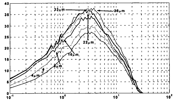
Fig. 3. Q vs Frequency for thick copper metal inductors.
